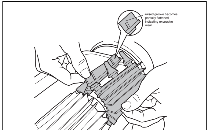
Figure 25. Worn Brush Indicator
