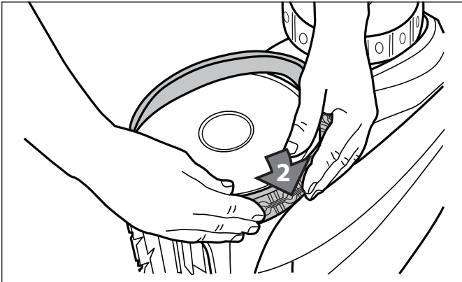
Figure 33. Start on One Side of the Tyre
