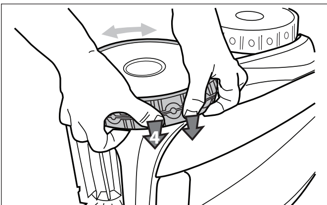
Figure 35. Push the Tyre into Place on the Wheel
