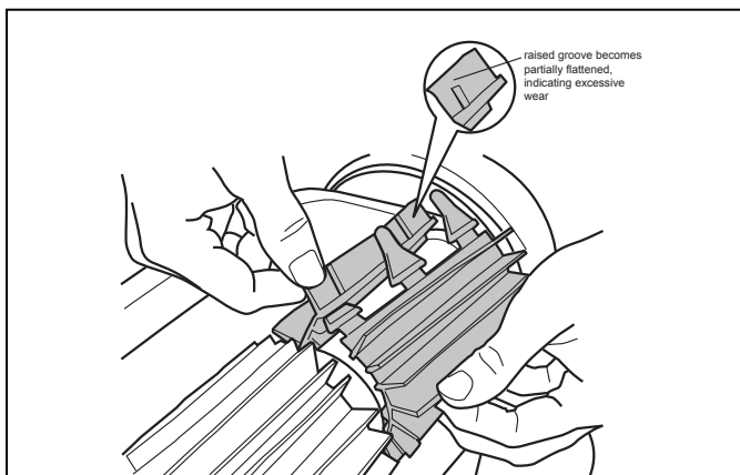
Figure 24. Worn Brush Indicator
